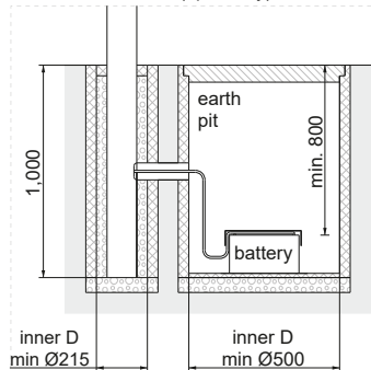
Sleeve foundation (optionally)
